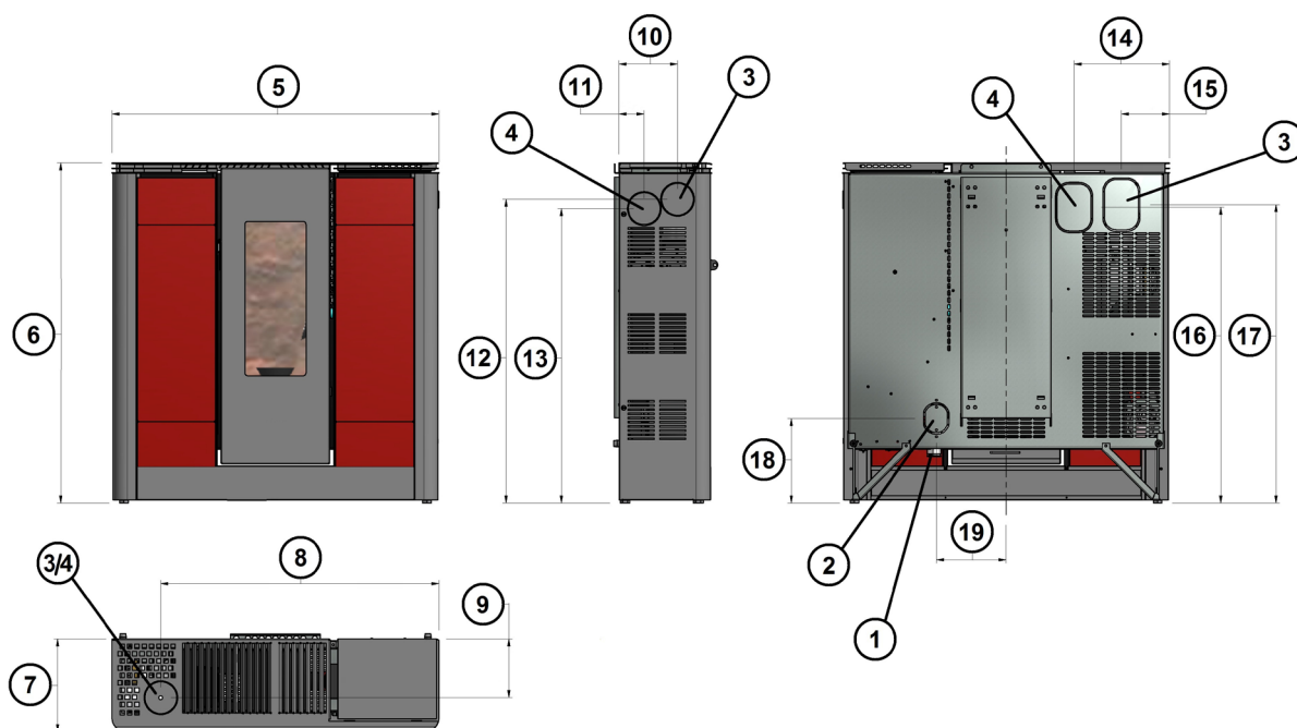
Fig. 13 - General dimensions: Style
