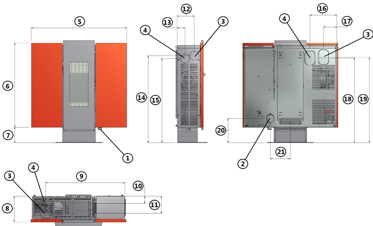
Fig. 12 - General dimensions: Wall/Small
