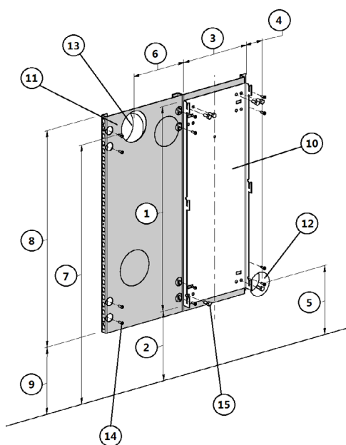
Fig. 17 - Mounting on flammable wall
