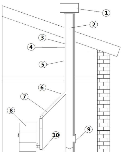
Fig. 5 - Chimney components
