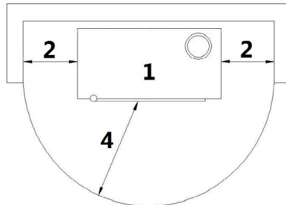
Fig. 15 - Wall mounting
