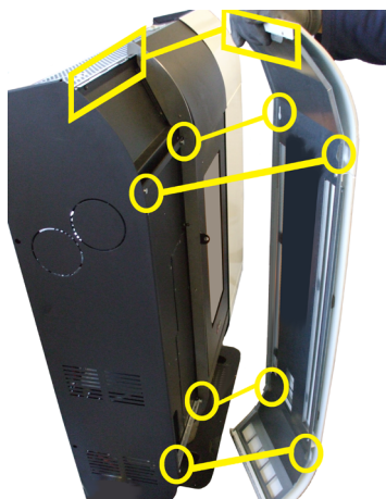
Fig. 20 - Panels assembly
