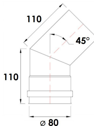
Fig. 16 - Curve at 45°
