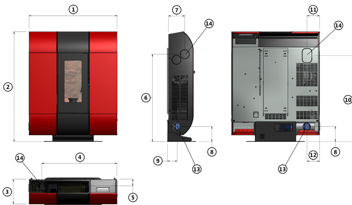
Fig. 11 - General dimensions
