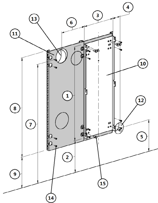
Fig. 19 - Mounting on flammable wall
