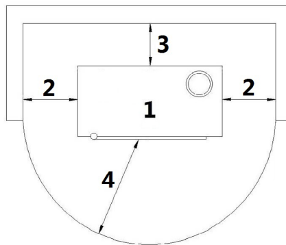
Fig. 14 - General installation with pedestal
