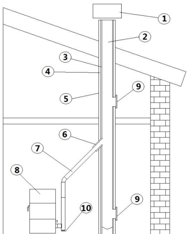
Fig. 5 - Chimney components
