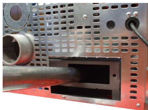
Fig. 38 - Fume chamber cleaning
