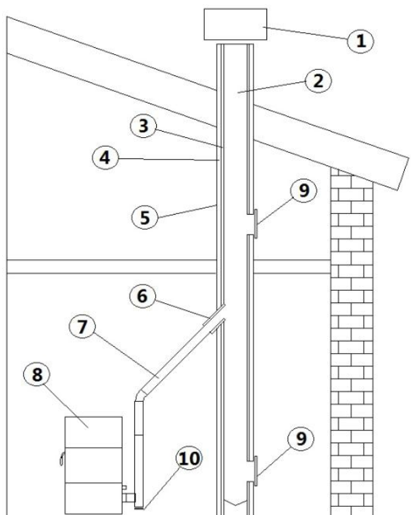
Fig. 5 - Chimney components
