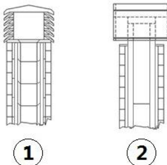
Fig. 4 - Anti-wind chimney pots
