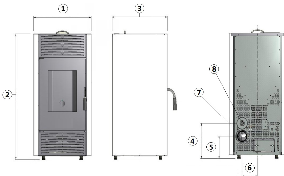
Fig. 11 - General dimensions
