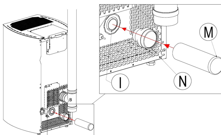
Fig. 8 - Anschlüsse
